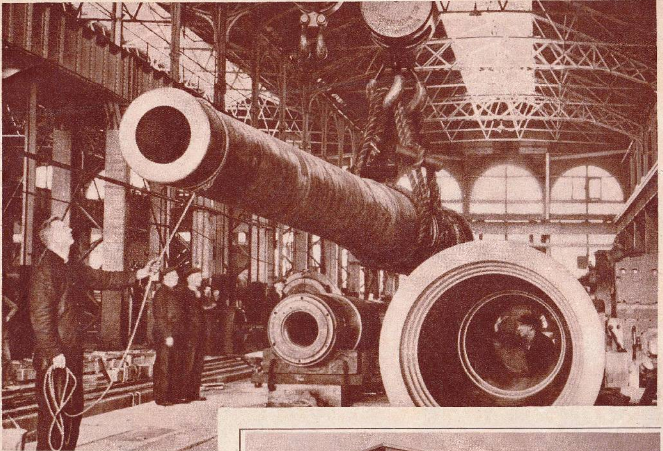
GUNS FOR THE BRITISH NAVY are made at the great Woolwich arsenal. Above: A huge gun is lifted by a travelling crane. Note the rifling visible at the muzzle. Below: A 16-inch gun has its firing chamber drilled out
